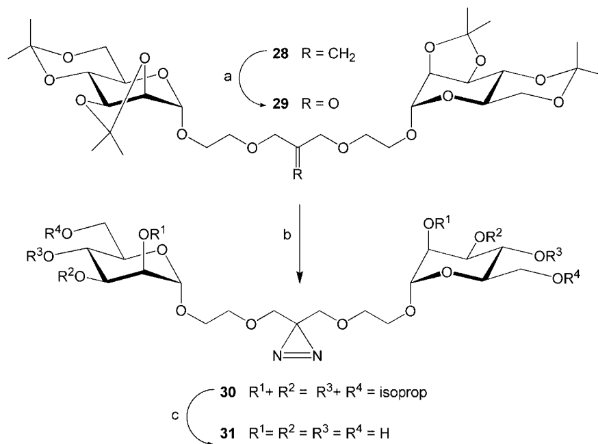
Scheme 4. a) \text{O}_3 , MeOH/dichloromethane, -78^\circ\text{C} , 20 min; then \text{PPh}_3 , 92%. b) \text{NH}_3 , \text{H}_2\text{NOSO}_3\text{H} , MeOH/dichloromethane, -50^\circ\text{C} \rightarrow -20^\circ\text{C} , 16 h; then 10% \text{I}_2/\text{MeOH} , TEA, 0^\circ\text{C} , 49%. c) TFA / \text{H}_2\text{O} , room temp., 10 min, 93%.
