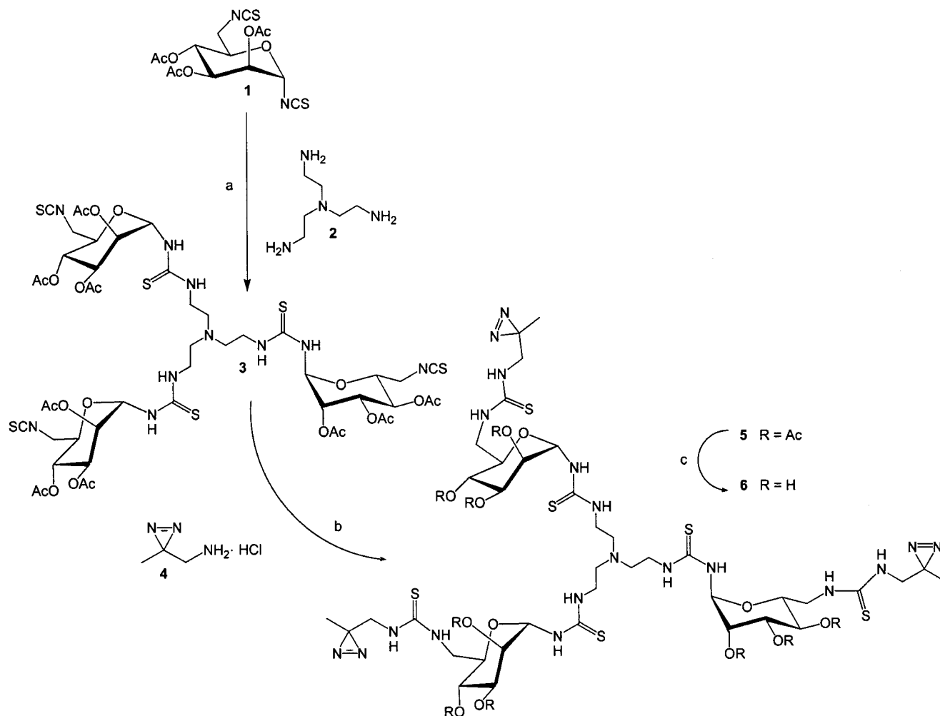
Scheme 1. a) Dichloromethane, 0 °C, 2 h, 70%; b) dichloromethane, DIPEA, room temp., 2 h, 52%; c) 1 M NaOMe in MeOH, 0 °C, 1 h, 69%.
