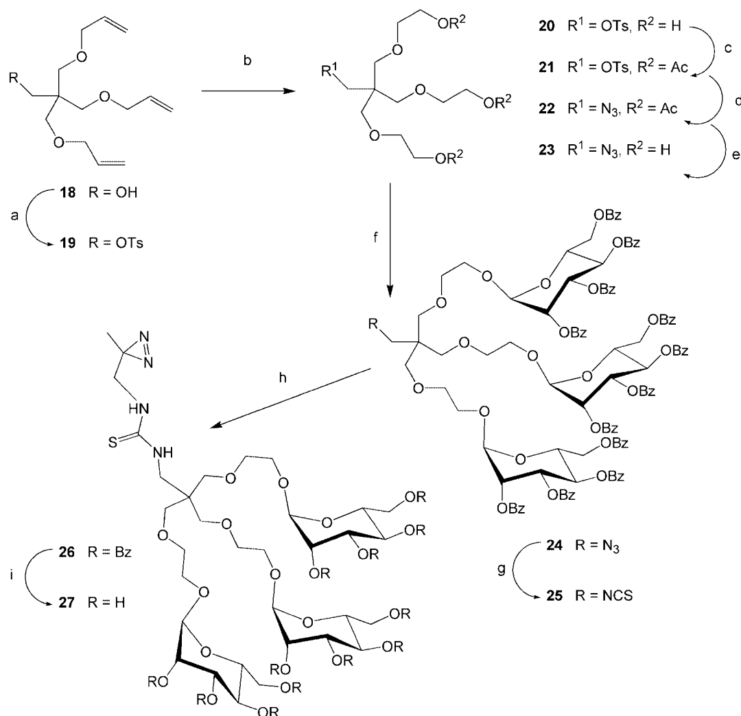
Scheme 3. a) TsCl, pyridine, room temp., 16 h, 81%. b) O 3 , MeOH, –78 °C, 0.5 h; then NaBH 4 , 46%. c) Ac 2 O, pyridine, room temp., 16 h, 84%. d) NaN 3 , TBABr, DMF, 80 °C, 6 d, 93%. e) 1 M NaOMe in MeOH, room temp., 0.5 h, 91%. f) 9 , TMS-OTf, dichloromethane, Ar, 0 °C → room temp., 1 d, 67%. g) CS 2 , P(OEt) 3 , toluene, 80 °C, 8 h, 83%. h) 4 , DIPEA, dichloromethane, 30 °C, 8 h, 80%. i) 1 M NaOMe in MeOH/THF, room temp., 1 h, 55%.
