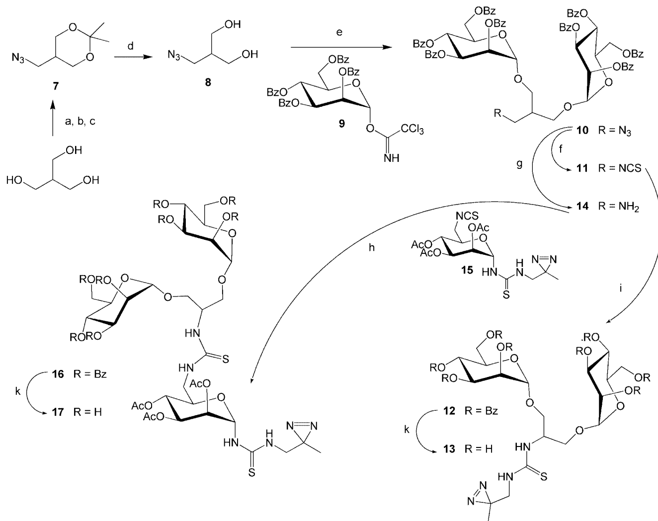
Scheme 2. a) DMP, acetone, TsOH, THF, room temp., 1.5 h; then b) TsCl, pyridine, room temp., 12 h; then c) NaN 3 , TBABr, toluene, 60 °C, 24 h, 41% over three steps. d) HCl, MeOH, room temp., 1 h, quant. e) TMS-OTf, dichloromethane, Ar, 0 °C → room temp., 1 d, 75%. f) CS 2 , P(OEt) 3 , toluene, 80 °C, 8 h, 56%. g) PPh 3 , THF, Ar, 0 °C → room temp., 1 h; then h) H 2 O, 23% over two steps. i) 4, DIPEA, dichloromethane, room temp., 2 h, 48%. k) 1 M NaOMe in MeOH/THF, room temp., 1 h, 65% for 13 ; 63% for 17 .
